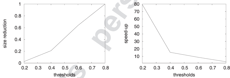
Fig. 4. Size reduction and speed-up from Table 4.
