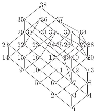
Fig. 1. Concept lattice \mathcal{B}(X, Y, I) of data table from Table 1.
