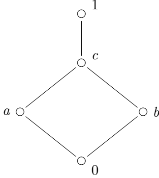
Figure 1: Residuated lattice from the proof of Proposition 6.
